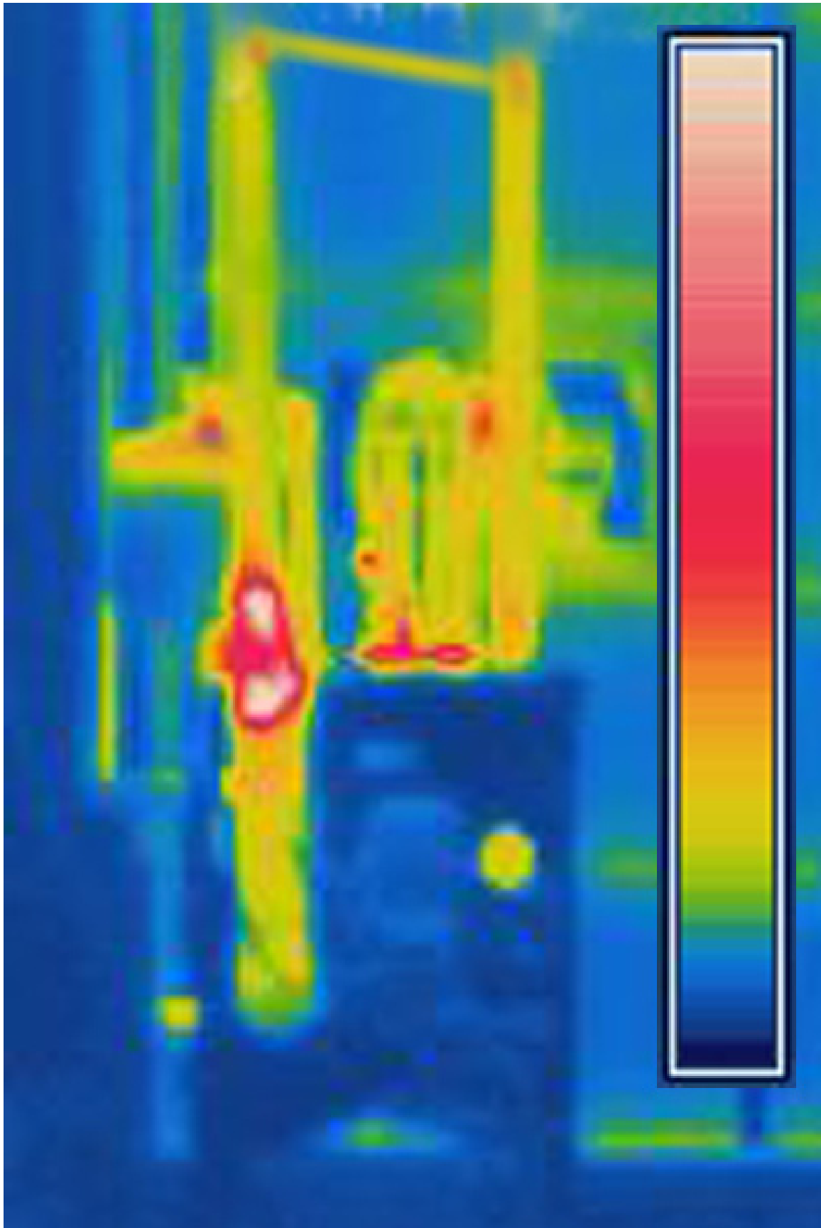
INFRARED IMAGE OF HOT WATER BOILER WITH THE BOILER JACKET™ KIT INSTALLED
